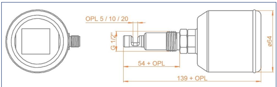
Fig. 1: Sensor dimensions
